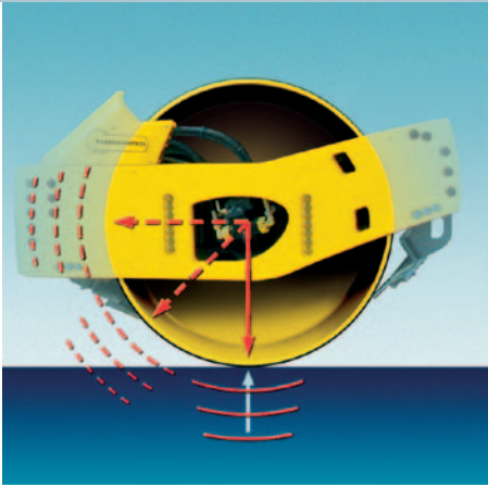
BOMAG VARIOCONTROL: lineare Vibration ...
